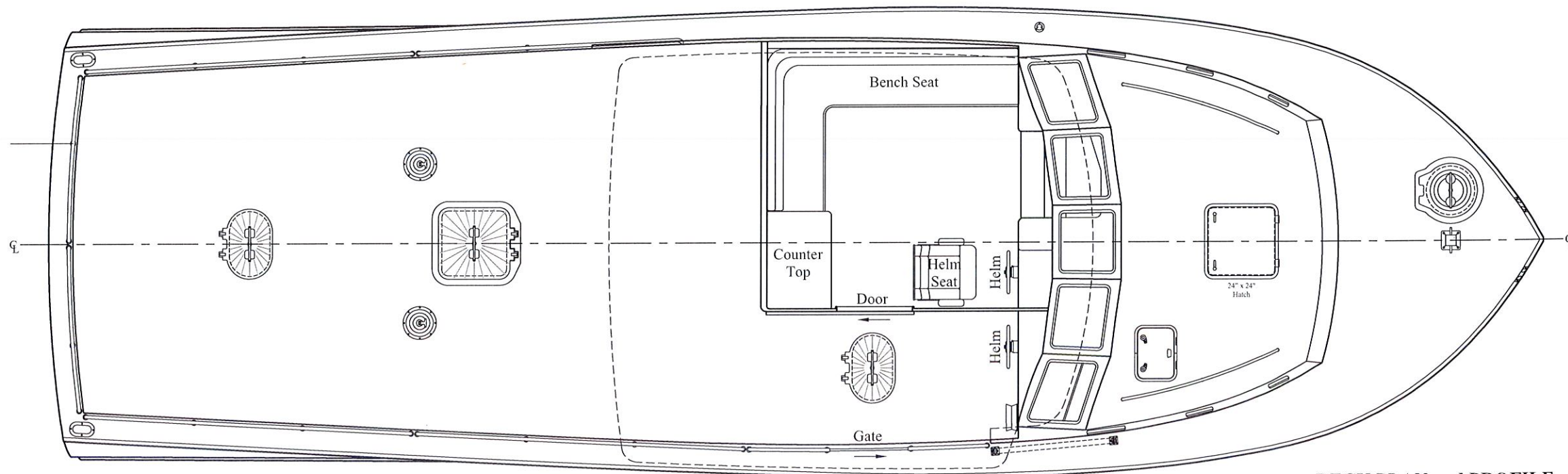
DECK PLAN and PROFILE Wesmac 46 - 46100
